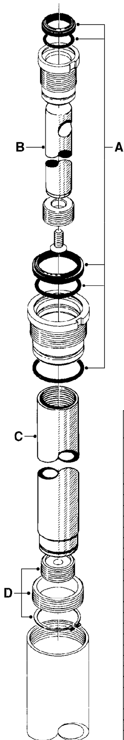
MULTI-STAGE CYLINDER
