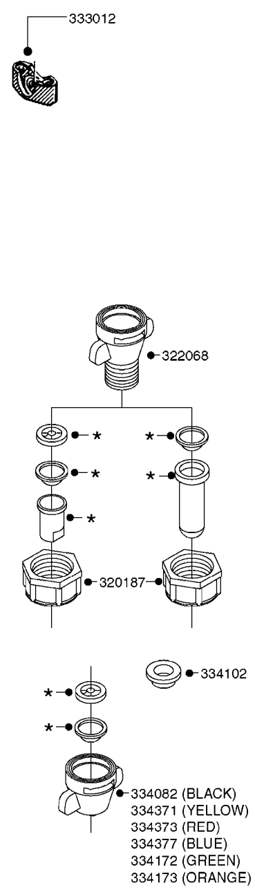
SINGLE NOZZLE BODY
